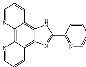
MePhenImPy: 1-methyl-2-(2-pyridyl)imidazo[4,5-f]-[1,10]phenanthroline (5)
