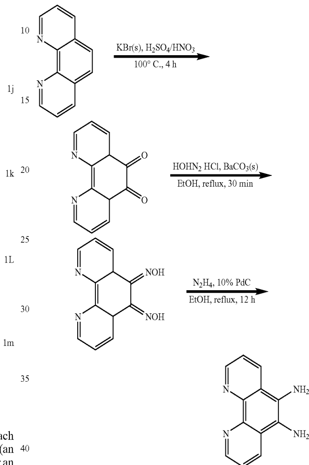
Scheme 1. Preparation of precursors for Scheme 2.
