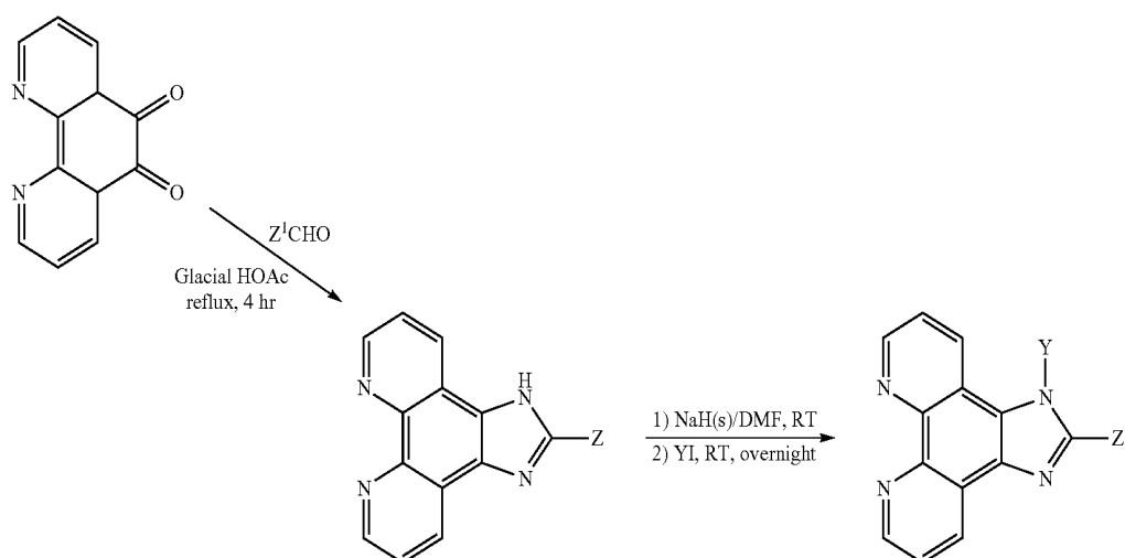
Scheme 2. Preparation of compounds of the general formula (1).
