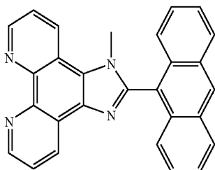
MePhenImAn: 1-methyl-2-(9-anthryl)imidazo[4,5-f]-[1,10]phenanthroline (3)
